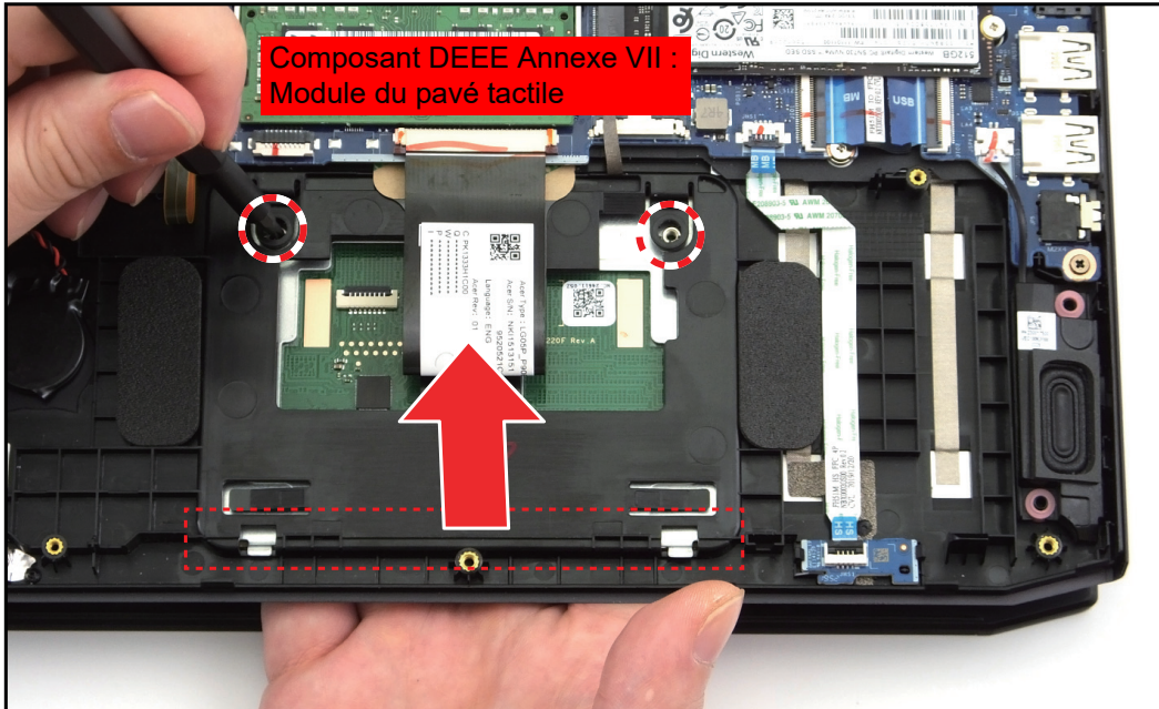
Figure 1-34. Retirer le pavé tactile
