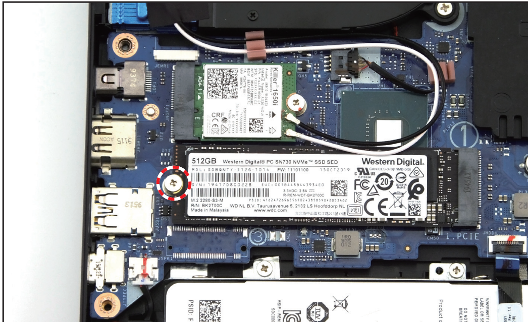
Figure 1-13. Retirer la vis
